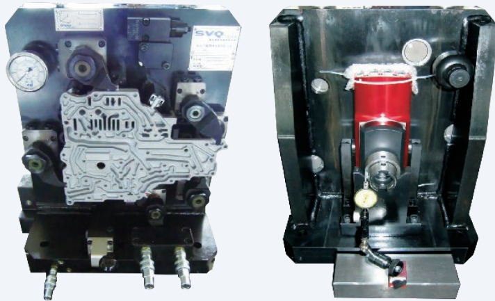
阀体夹具 Valve Body Fixture
