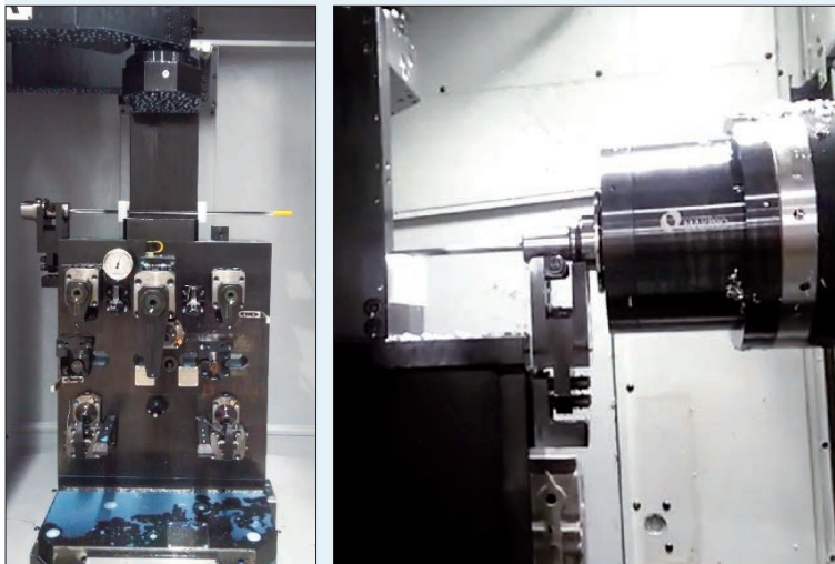
阀体夹具 Valve Body Fixture
